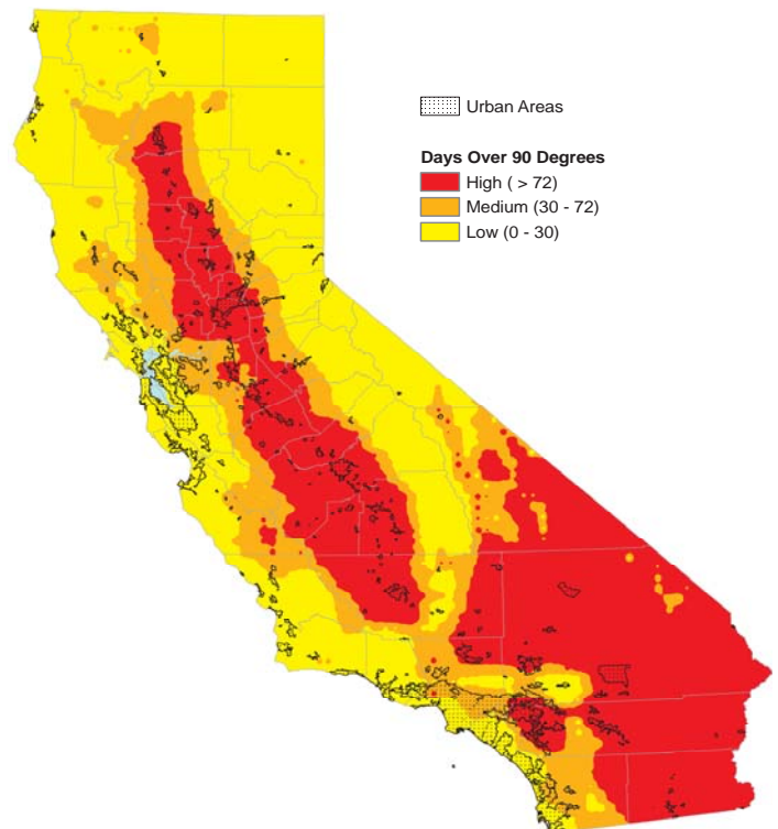
Figure 3.2.1. California urban areas by annual average days over 90 °F. Data Sources: Daily Temperatures, California Climate Action Team (2008); Urban Areas, U.S. Census Bureau (2000); USGS National Land Cover Dataset (2001)
