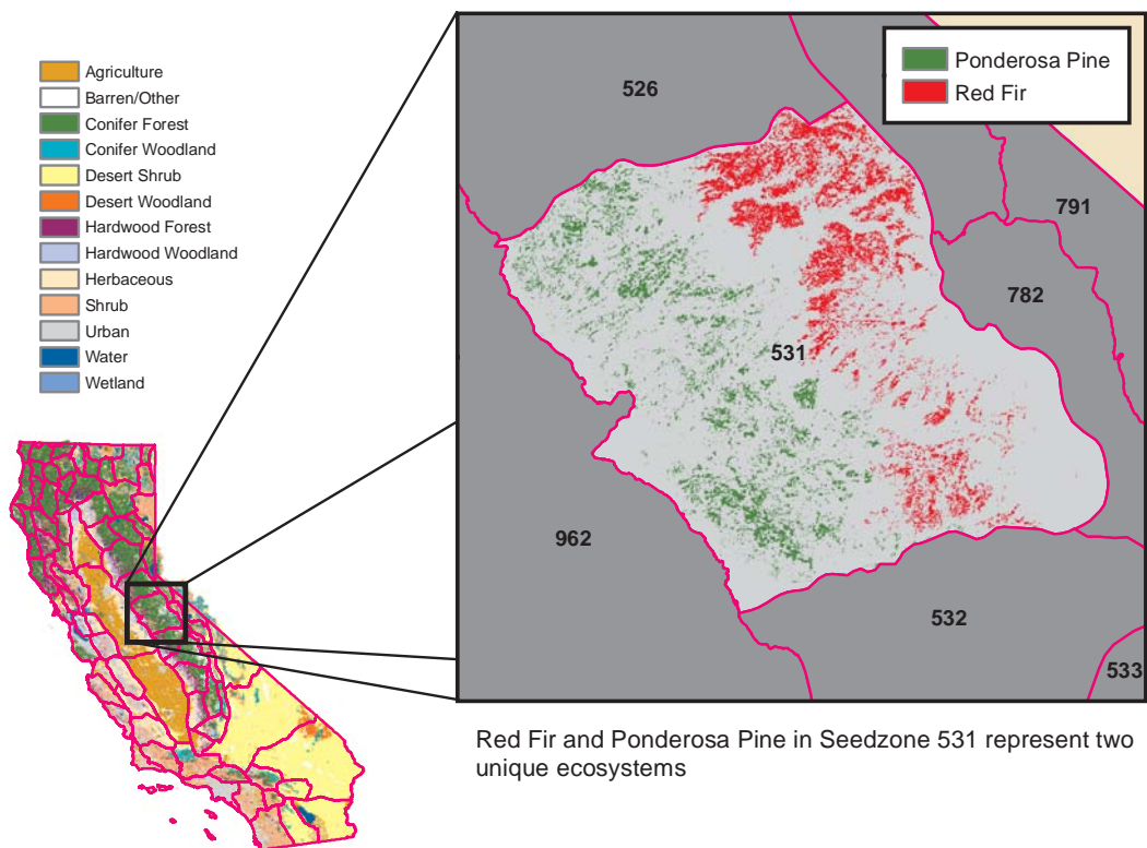
Figure 2.2.3. Land cover and tree seed zones in California.
