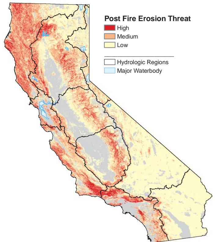
Figure 3.1.11. Post-fire erosion threat. Soil erosion following wildfires can accelerate sediment delivery to stream courses and through siltation can impact to water storage facilities. Data Sources: Post-Fire Erosion Potential, FRAP (2004); Fire Threat, FRAP (2005); Statewide Land Use / Land Cover Mosaic, FRAP (2006) Watershed Boundaries Database for California, NRCS (2009)
