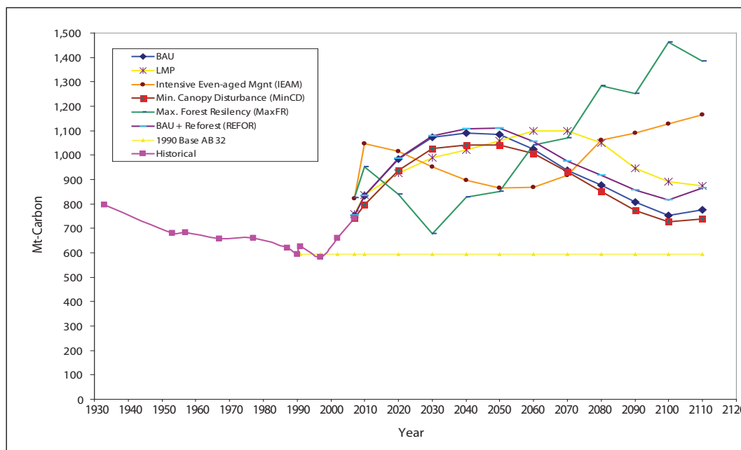
Figure 1.2.1. Results from U.S. Forest Service analysis of projected carbon stocks on national forests in California. Source: Goines and Nechodom, 2009
