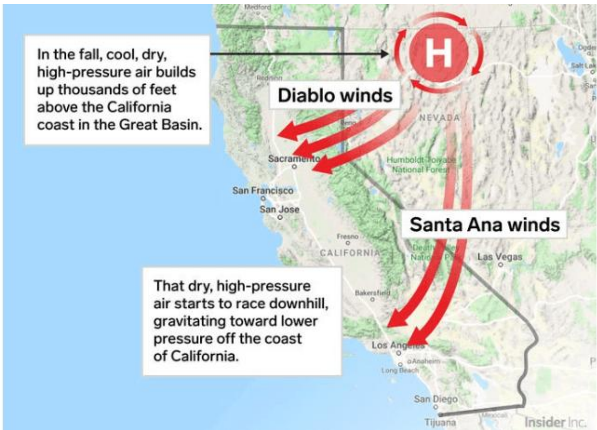
Figure 5. Illustration and explanation of the Diablo and Santa Ana winds. Source Weather Gamut .
