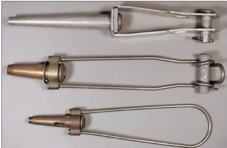
Figure 3-67 Automatic Deadends
