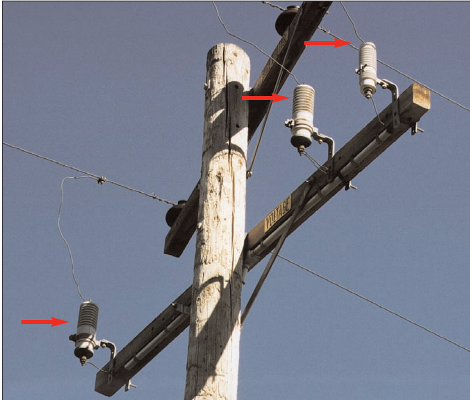
Figure 2-21 Lightning Arrester
