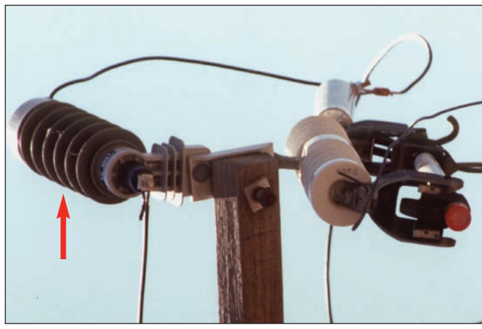
Figure 2-23 Non-Porcelain Lightning Arrester
