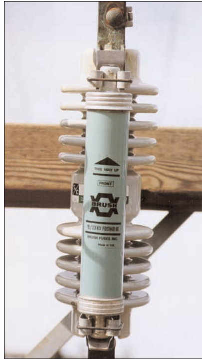
Figure 3-2 Arm Mounted Cutout with Non-Expulsion Fuse
