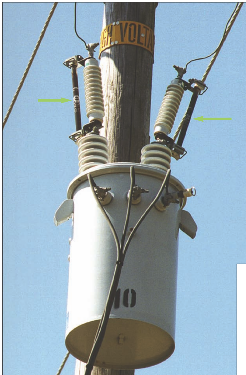
Figure 3-12 Over head Conventional Transformer with Bushing Mounted Cutout and Liquid Filled Fuse
