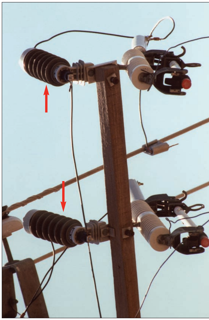
Figure 2-24 Non-Porcelain Lightning Arrester
