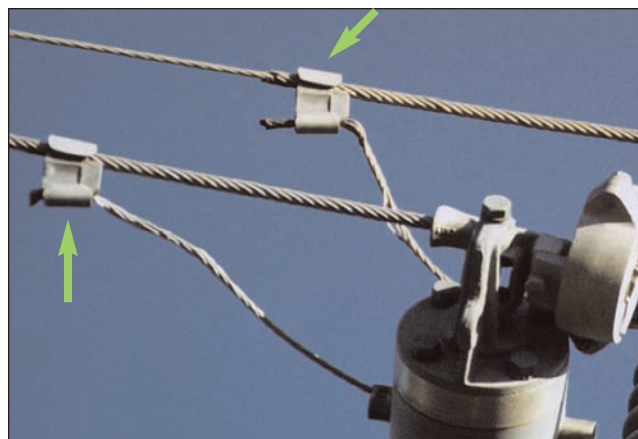
Figure 3-60 Fired Wedge Connectors on Line
