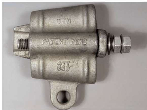
Figure 3-59 Bolted Wedge Connector
